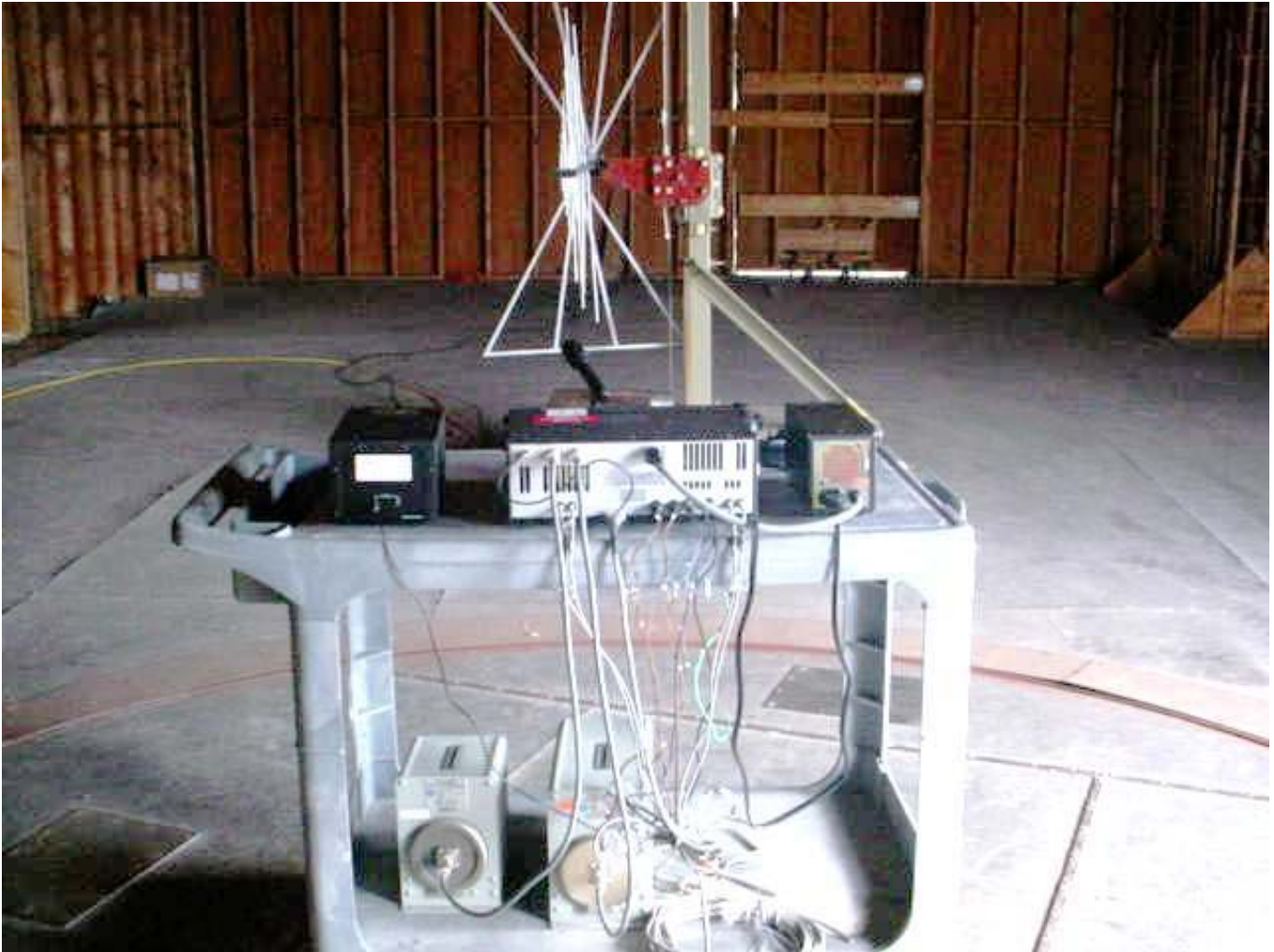
Radiated Emissions at 3 Meters (Rear View)
